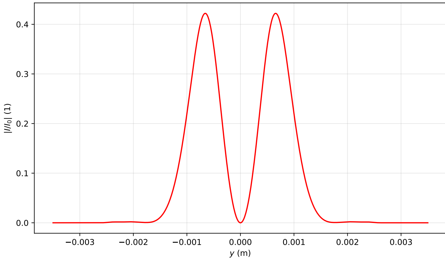
Intensity profile I(x=0, y, z=2.070)/I_0 , P_{in}=3.0P_{cr} , artificial time
